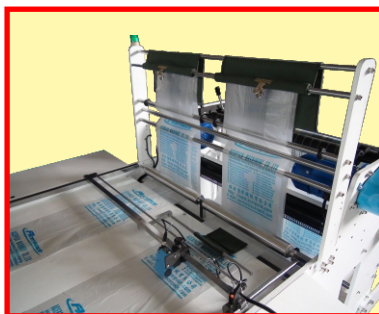
In-feed guide device
