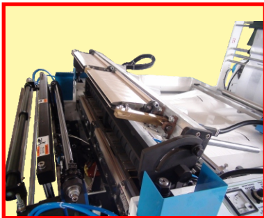
Turn-up sealing design
